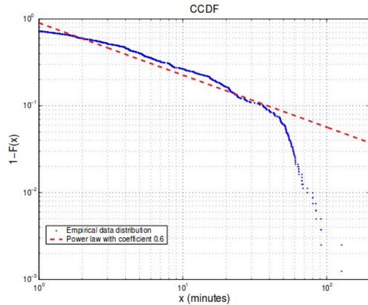
Fig. 8. Pairwise contact time distribution (log scale).
